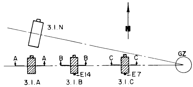
KEY PLAN
